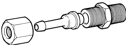
Nipple R 1 / 4 x G 3 / 8 A cone (brass)
